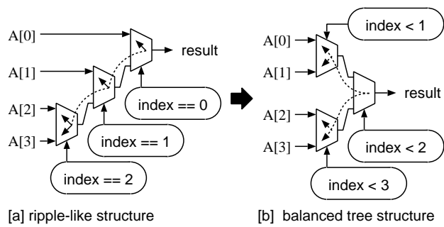
Figure 12. RegArr reading implemented via a balanced tree.
